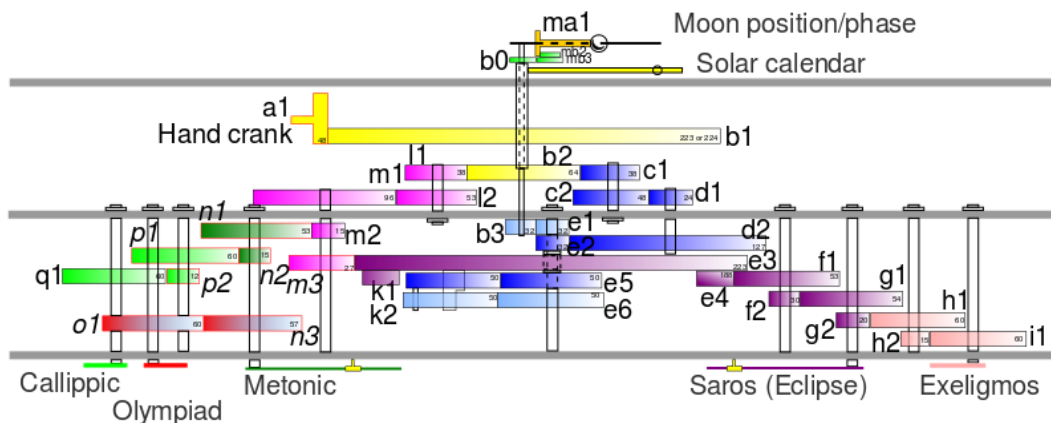
Figure 1.2: The Antikythera Mechanism: gear chain diagram for the known elements of the mechanism. Hypothetical gears in italics. From http://en.wikipedia.org/wiki/Antikythera_mechanism . ©Lead holder / Wikimedia Commons / CC BY
