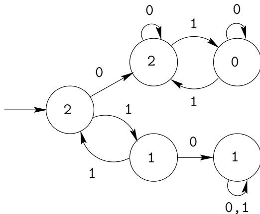
Fig. 2. Automaton generating a squarefree sequence
