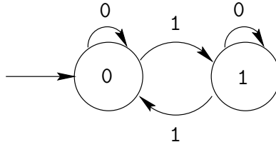
Fig. 1. Automaton generating the Thue-Morse sequence
