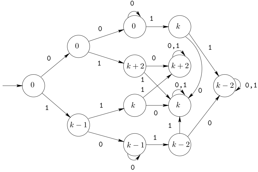
Fig. 4. Automaton generating the continued fraction for \alpha_k
