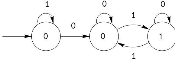
Fig. 3. Automaton generating the lexicographically least sequence in the orbit closure of the Thue-Morse sequence
