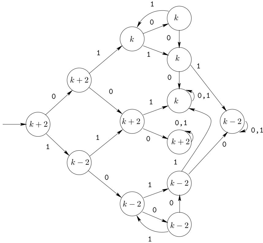
Fig. 5. Automaton generating the continued fraction for \zeta_k
