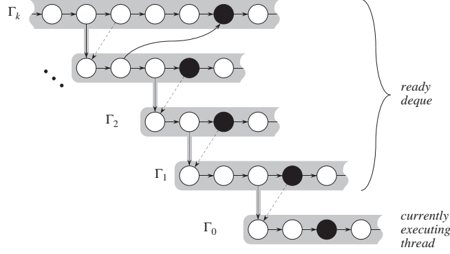
Figure 3: The structure of a processor’s ready deque. The black instruction in each thread indicates the thread’s currently ready instruction. Only thread \Gamma_k may have been worked on since it last spawned a child. The dashed edges are the “deque edges” introduced in Section 6.
