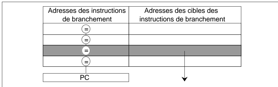
Figure 6.25: Principe du cache de branchements
