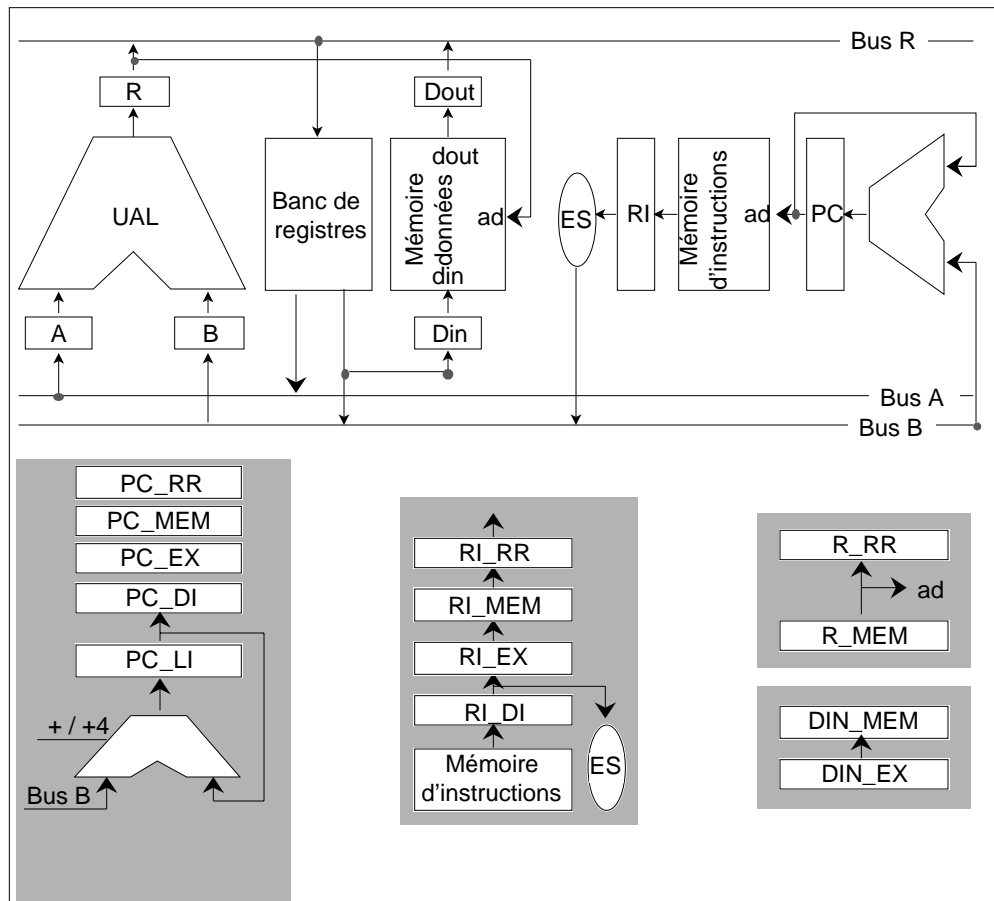
Figure 6.20: Microarchitecture pipelinée
