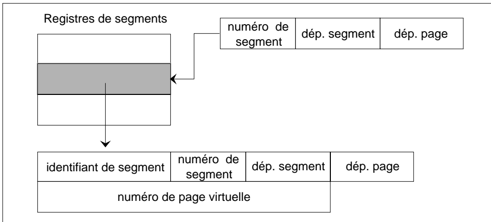
Figure 8.10: Segmentation paginée
