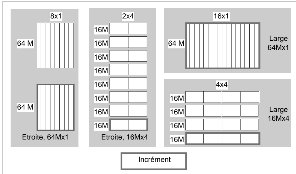
Figure 7.18: Incrément mémoire
