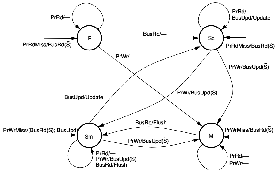
Figure 2 : protocole DRAGON
