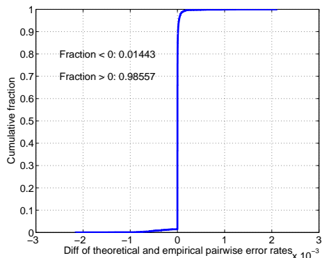
Fig. 6. Pairwise Host Error Rates
