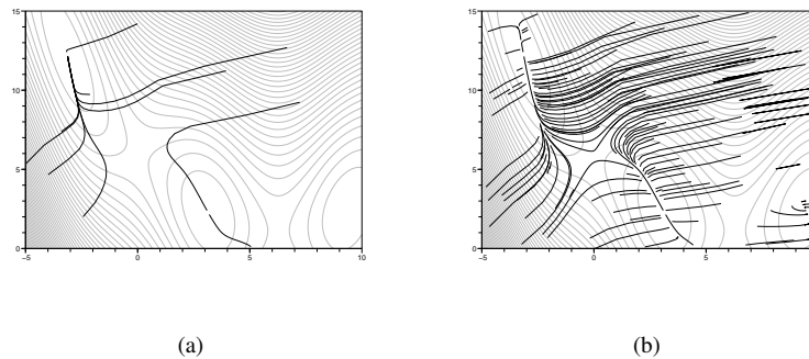
Figure 14.4. Multistart optimization strategies. In (a), different runs are performed independently of each other. In (b), the optimization trajectory is interrupted when it meets that of a precedent run; a new run begins in a different region of the domain.
