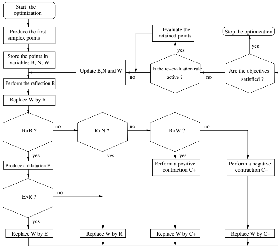
Figure 14.9. Flow chart of the simplex method algorithm.
