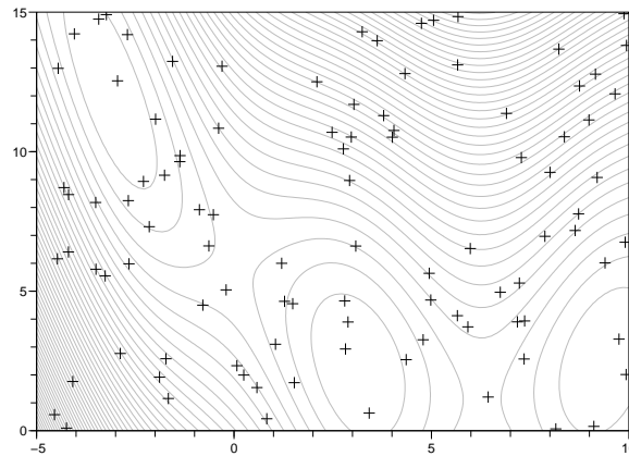
Figure 14.5. Sample run of the rsearch optimizer with 100 iterations on the Branin-Hoo function.
