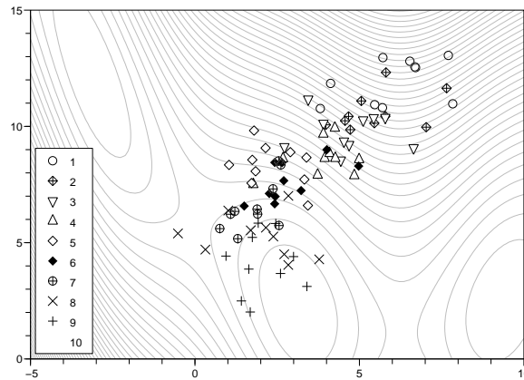
Figure 14.6. Example of a muLambda optimizer (evolution strategy (\mu/\mu, \lambda) ) convergence on the Branin-Hoo function with \mu = 2 parents, \lambda = 10 offsprings and 10 iterations (i.e., 100 evaluations in total).
