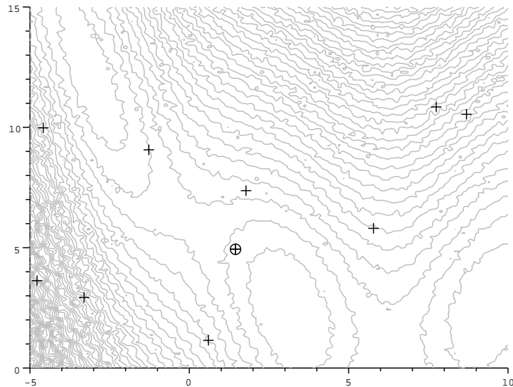
Figure 14.15. Example run of the Ask & Tell algorithm on an uncertain version of the Branin-Hoo function, 50 Monte Carlo simulations per point. The best point found after testing 10 points is enclosed within a circle. The contour lines were also calculated with 50 Monte Carlo simulation.
