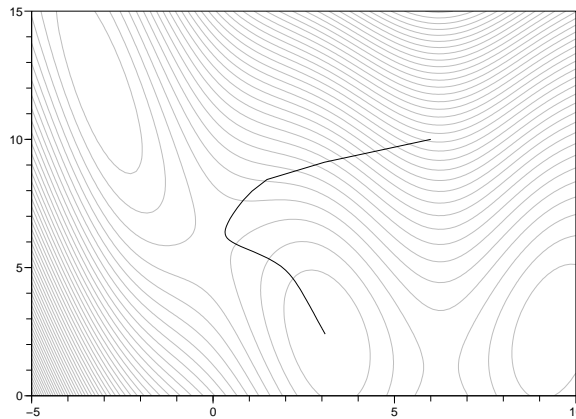
Figure 14.7. Example of a steepdesc execution with 100 iterations on the Branin-Hoo function.
