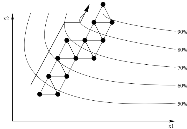
Figure 14.10. Path of a simplified simplex method (only reflections are made). The algorithm correctly finds an uphill direction (the function is maximized here).
