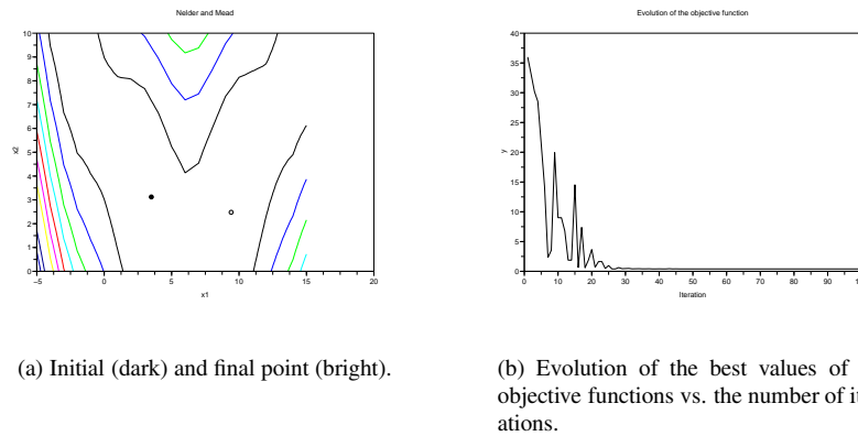
Figure 14.12. Example of a run of the Ask & Tell version of the Nelder & Mead algorithm on Branin's function.
