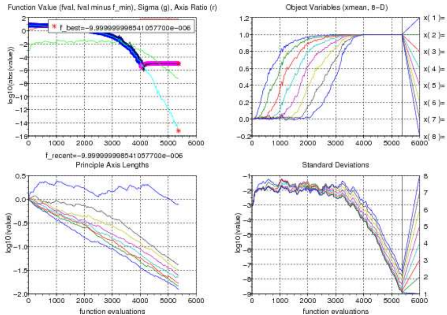
Figure 14.13. Output of cma_plot from an optimization run on the 8-D Rosenbrock function, where 10^{-5} was subtracted from the original function value. Upper left: The function value (thick line in blue and magenta) becomes negative after about 4000 function evaluations (400 iterations). The cyan line (final value 10^{-15} ) shows the difference to the best achieved function value and reveals a continuing improvement, as the line is decreasing until termination. Lower left: The principle axes lengths of the sample distribution (in log-scale) adapt to the minimized function. They reveal the (local) structure of the underlying optimization problem. Upper right: the variables move from zero to one in an ordered fashion. The global optimum is at x_i = 1 for all i = 1, \dots, 8 . Lower right: the standard deviations quickly increase during the first iterations by about one order of magnitude from 10^{-3} to 10^{-2} . They also vary during the optimization by a factor of about three and quickly decrease during the final convergence phase after 4000 function evaluations.
