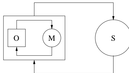
Figure 14.3. Example of an optimization procedure based on a metamodel. The group made of an optimizer and a metamodel yields a new optimizer which is coupled to a computationally expensive simulator. After each new simulation, the metamodel is updated. The solution point found by optimizing the metamodel is presented to the simulator at each outerloop iteration.
