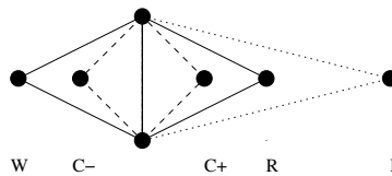
Figure 14.11. Expansion and contraction steps of the simplex method.
