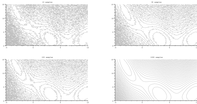
Figure 14.14. Effect of the number of Monte Carlo simulations on the average estimation of the Branin function with uncertainties. From left to right and top to bottom, 10, 30, 100 and 1000 samples.
