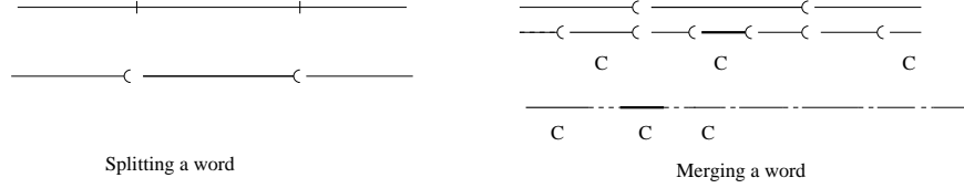
Fig. 2. The correction (steps 1.a and 1.b) of a word with two infeasible subwords where C is some connected components (and h' = 3 for the proof of Lemma 2).
