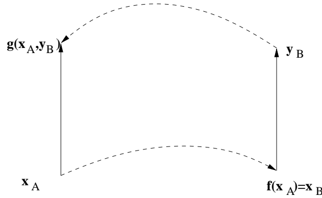
FIGURE 17.3. Lin -reduction between two optimization problems.
