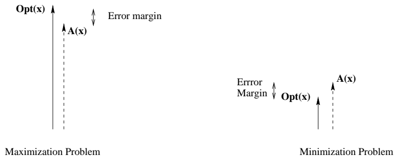
FIGURE 17.1. Approximation of a maximization or minimization problem.
