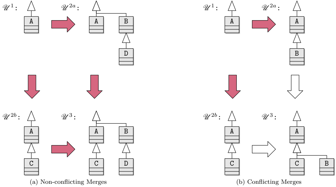
Figure 4. Merging Universes: Figure 4a illustrate the non-overlapping extension of a class A with one direct subclass C and a new hierarchy consisting of the classes B and D which are rooted on the same level as A. In contrast, Figure 4b illustrates a conflicting merge. In this case, the class A is extended independently with the direct subclasses B and C which causes a conflict when merging these two extensions.
