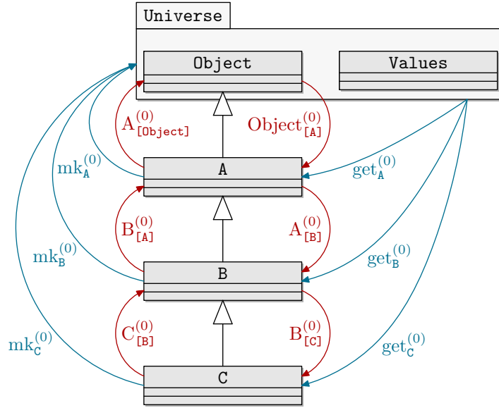
Figure 3. The type casts, e.g., B_{[C]}^{(0)} allow the conversion of a type to its direct successor or predecessor in the type hierarchy. The injections, e.g., mk_B^{(0)} convert a class type to the universe type and the projections, e.g., get_B^{(0)} , convert a universe type to a concrete class type. For a universe without values, the class type and the universe type of the top most class are identical. Here, the package Universe represents the universe, i.e., the top level class ( Object ) and the primitive types ( Values ).
