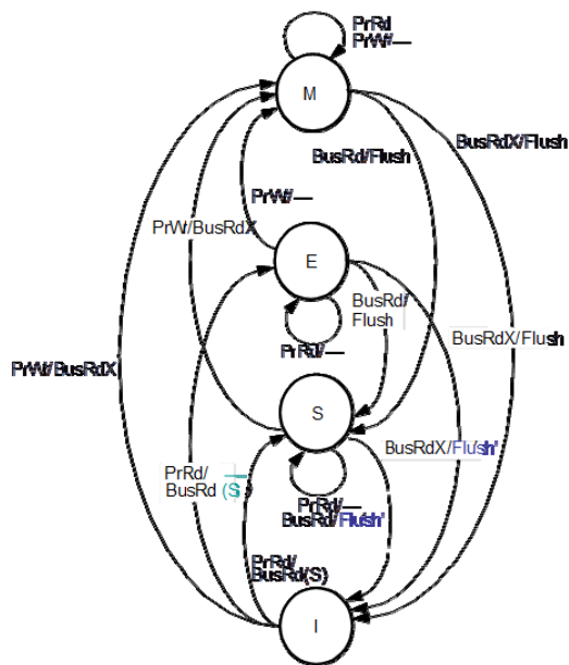
Figure 4 : protocole MESI
