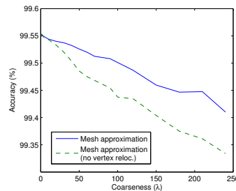
Fig. 8: Approximation with and without vertex relocation.
