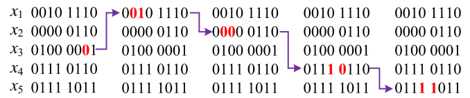
Fig. 8. The bitmasks used in P2P. There are five tags and we present the first two words of EPCs in binary. we can first set the bitmask BM = (000_2, 6, 1, 0_2) to query tag x_3 , then use BM = (000_2, 1, 2, 01_2) , BM = (000_2, 1, 2, 00_2) , BM = (000_2, 3, 2, 10_2) , BM = (000_2, 3, 2, 11_2) in sequence to query tags x_1, x_2, x_4, x_5 , respectively.
