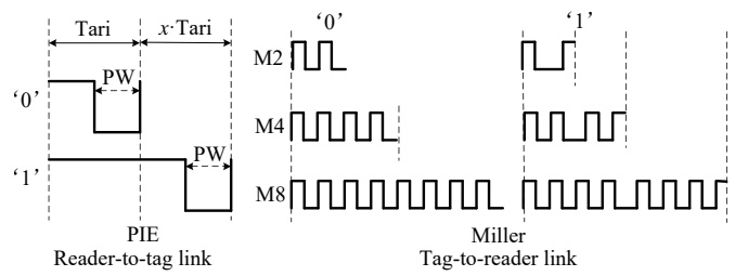
Fig. 2. Data encoding in the Gen2 standard.
