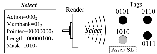
Fig. 6. Illustration of a selective query in P2P. There are four tags with EPCs: 0101, 0110, 1010, 0111, respectively. With the configuration: Action=000 2 , Membank=01 2 , Pointer=00000000 2 , Length=00000100 2 , Mask=1010 2 , the reader asks the tags to compare the bit string from the 1-st to the 4-th bit in their individual EPCs with the content in Mask of the received Select 5 .
