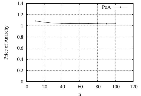
Fig. 3. System efficiency at the correlated equilibrium
