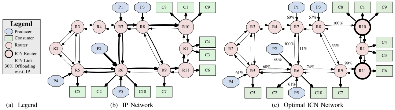
Figure 2. Example Scenario. We consider the Abilene topology with \alpha = 0.8 and budget of B = 3.5 \max_p . Fig. 2b represents the IP network, while Fig. 2c is the solution of the optimal ICN planning. The overall cost for the IP network is 14.3 \cdot 10^6 USD, while in the optimal ICN network it decreases to 7.6 \cdot 10^6 USD. Line size is proportional to the aggregate traffic the link is transferring, while the link offloading percentage reported in Fig. 2c compares the traffic in ICN w.r.t. the one of the IP network.
