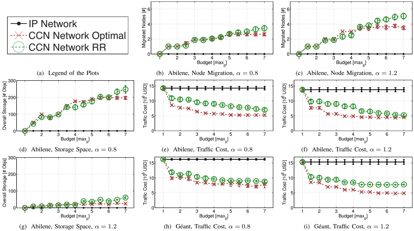
Figure 3. Effect of the Budget . Fig. 3a is the common legend of all the plots. Fig. 3b-3g are relative to the Abilene topology, while Fig. 3h,3i refer to Géant. The number of ICN migrated routers is shown in Fig. 3b,3c for different \alpha values, similarly, the overall storage is plotted in Fig. 3d,3g. Lastly, the traffic cost component is depicted in Fig. 3e, 3f for Abilene, and in Fig. 3h,3i the traffic in Géant is available.
