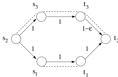
Fig. 1. Hexagon network topology: the 3 players must connect their source-destination nodes (s_i, t_i) . The optimal solution, which in this case coincides with both the Nash equilibrium point and the Nash bargaining solution, is illustrated with dashed lines.
