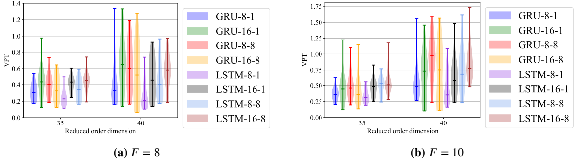
Figure 23: Violin plots of the VPT in the testing data for stateful LSTM and GRU models trained with different truncated Backpropagation through time parameters \kappa_1 and \kappa_2 in the (reduced) SVD mode observable of the Lorenz-96 system. The legend of each plot reports the models along with their \kappa_1 - \kappa_2 parameters used to train them. The three markers report the minimum, mean and maximum VPT. We observe that especially in the reduced order observable scenario ( d_0 = 35 ), having a large truncated back-propagation parameter \kappa_1 (also referred to as sequence length) is vital to capture the temporal dependencies in the data and achieve high forecasting efficiency. In contrast in the full-state scenario ( d_0 = 40 ) a model with a small back-propagation horizon suffices.
