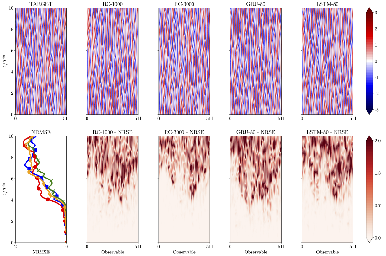
Figure 14: Contour plots of a spatio-temporal forecast starting from an initial condition in the testing dataset with parallel GRU, LSTM, and RC networks along with the true (target) evolution and the associated NRSE contours in the Kuramoto-Sivashinsky equation with the full state as an observable d_o = 512 . The evolution of the component average NRSE (NMRSE) is plotted to facilitate comparison.
