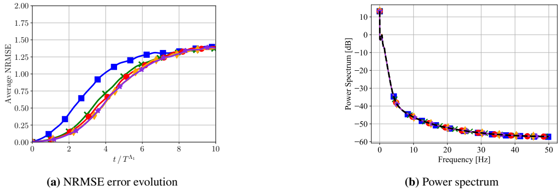
Figure 10: (a) The evolution of the NRMSE error (averaged over 100 initial conditions) of different parallel models in the Lorenz-96 with state dimension d_o = 40 . (b) The reconstructed power spectrum. All models accurately capture the power spectrum. RCs with d_h \in \{6000, 12000\} nodes are needed to match the predictive performance of an LSTM with 100 nodes. RC-1000 \blacksquare ; RC-6000 \blacktriangleright ; RC-12000 \blacklozenge ; GRU-500 \blacklozenge ; LSTM-100 \blacktriangleleft ; Groundtruth -\cdot-\cdot ;
