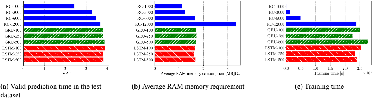
Figure 9: (a) Valid prediction time (VPT), (b) CPU memory utilization and (c) total training time of RNN parallel architectures with group size G = 2 and an interaction length I = 4 forecasting the dynamics of Lorenz-96 with state dimension d_o = 40 (full state). GRU and LSTM results do not depend significantly on network size. RC with 3000 or 6000 nodes have slightly lower VPT, but require much less training time. Increasing RC size to more than 12000 nodes was not feasible due to memory requirements.
