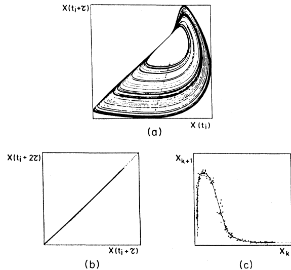
FIG. 9. Experimental plot of a Poincaré section in the Belousov-Zhabotinski reaction, after Roux and Swinney (1981): (a) the attractor and the plane of Poincaré section; (b) the Poincaré section; (c) the corresponding first return map.
