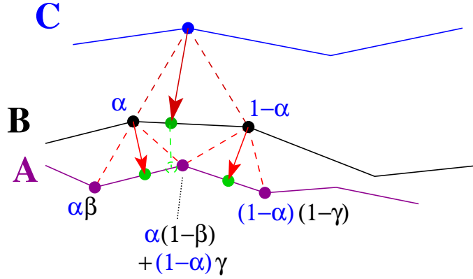
Figure 16: Simple case: compute the barycenter of the barycenters...
