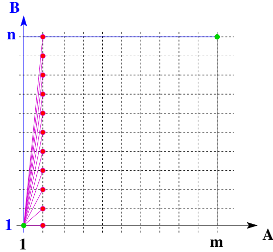
Figure 2: Compute the cost of all possible matchings for A_1 and A_2 .
