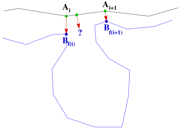
Figure 12: In the general case, no matching extension is possible. Just refine the discretization step on A or oversample it.
