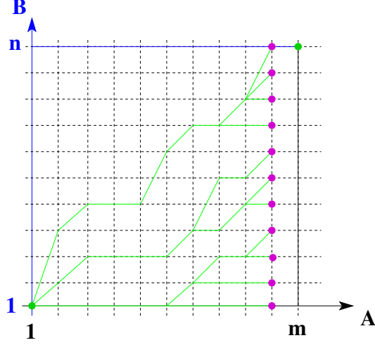
Figure 7: Best paths up to A_{m-1} , with associated costs C_{m-1}(f(m-1)) .
