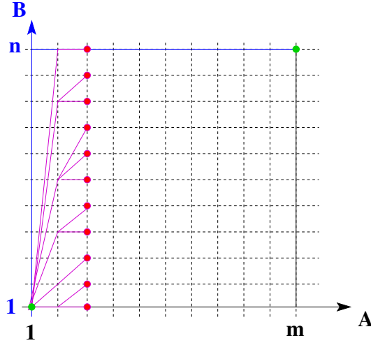
Figure 4: All best sequences of matchings up to A_j .
