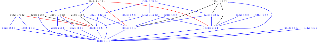
FIGURE 6. Graph encoding the characters of left and right class modules, and therefore the Cartan invariant matrix for M(\mathfrak{S}_4) . See the text for details.
