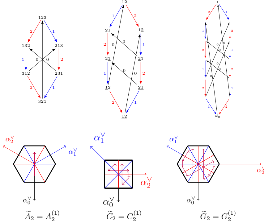
Fig. 1: Top: Graph of the action of \pi_0, \pi_1, \dots, \pi_n on the classical Weyl group \tilde{W} , using (signed) permutation notation. Bottom: The top graph can be realized geometrically by quotienting the alcove picture by the translations, or equivalently by identifying opposite edges of the "hexagons". An i -arrow in the graph corresponds to a negative i -crossing. The alcove walk goes from the antifundamental chamber w_0(A) back the fundamental chamber A .
