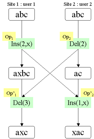
Figure 3. Counter-example violating condition C_1 .
