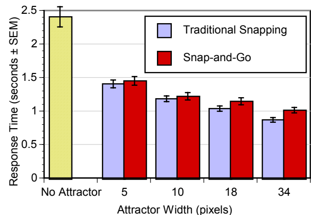
Figure 12: Task time by snapping technique and attractor width across all distances ( \pm standard error of the mean).
