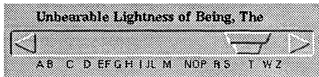
Figure 8: Redesigned Alphslider
