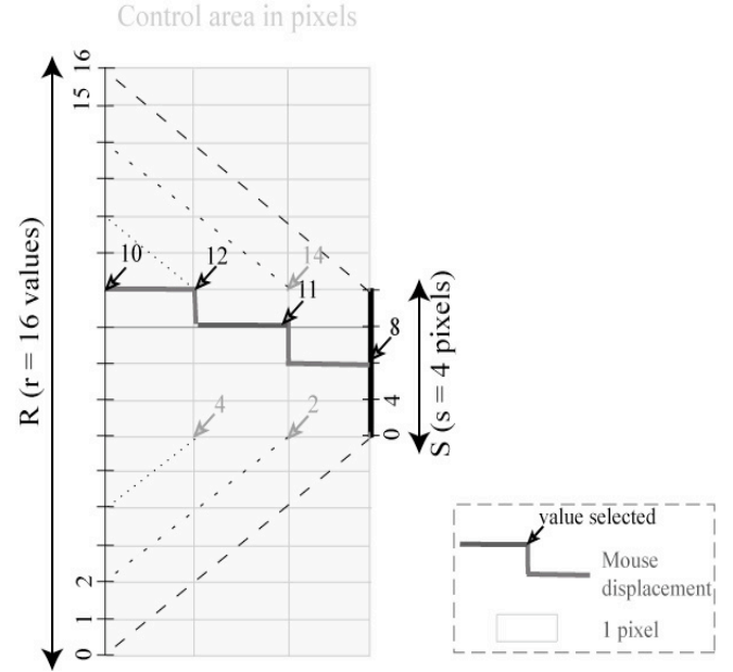
Figure 2: Using the orthogonal direction to adjust the control precision, i.e. the zoom level
