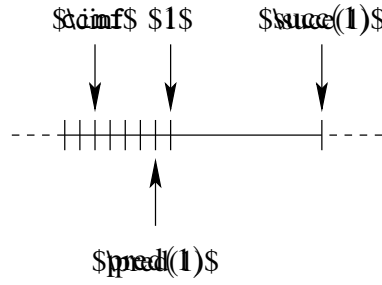
Fig. 2.1 Worst case for computing the predecessor in radix 10.
