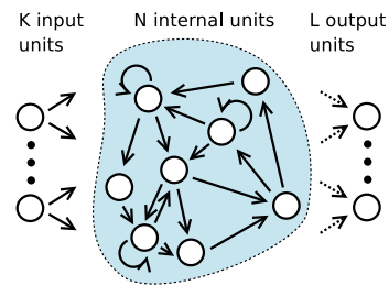
Fig. 5. Structure of an Echo State Network
